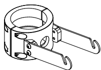
Braket \varnothing 76 l 150mm colour Graphite
